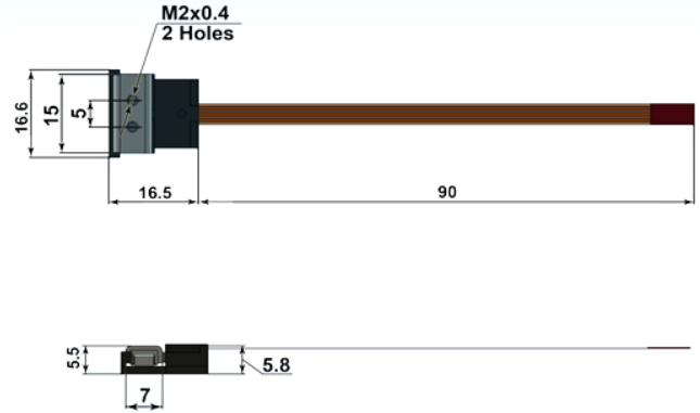
Schematic drawing (mm) of standard LRMO (without factory installed encoder).
