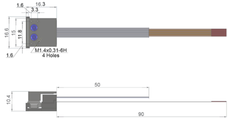
Schematic drawing (mm) of LRMO-E with factory installed encoder.
