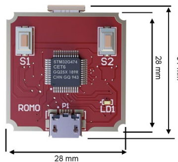
LRMO-E Electronic Driver PCB
